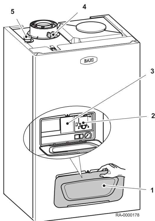
Fig.1 Oversigtsdiagram WGB-K EVO
